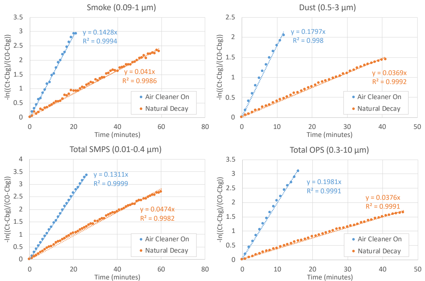
Figure 3. Estimated loss rate constants for four particle size ranges
